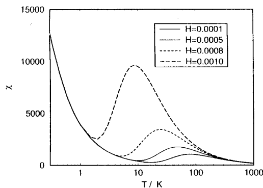
Fig. 4. Magnetic susceptibility \chi/\mu_B \frac{N}{V} at nonzero magnetic fields H ( \text{eV}/\mu_B ), for \Delta E = 0.01 eV, \mu_1 = 1.0 \mu_B , and \mu_2 = 10.0 \mu_B .
